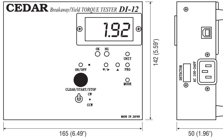
DI-12-SL02 detector
